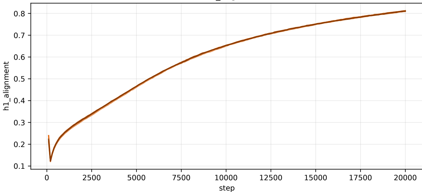
val/h1_alignment
