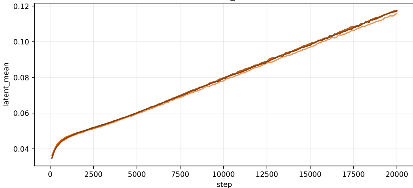
val/latent_mean
