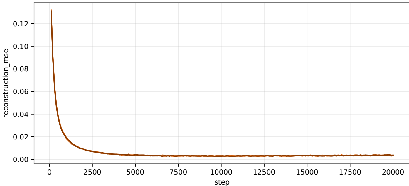
val/reconstruction_mse
