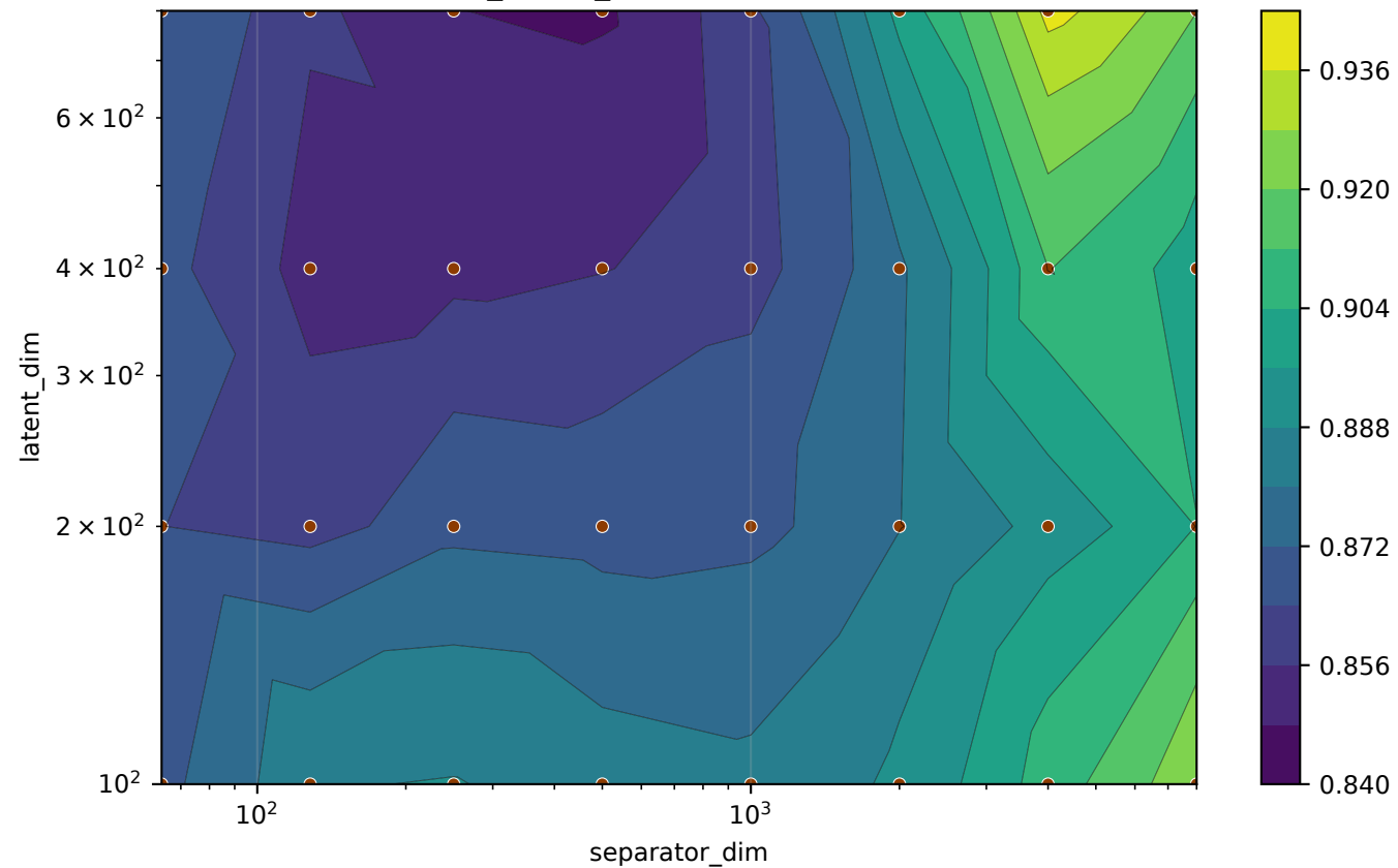
val/patterns_active_rate (steps=start..2000, last)
