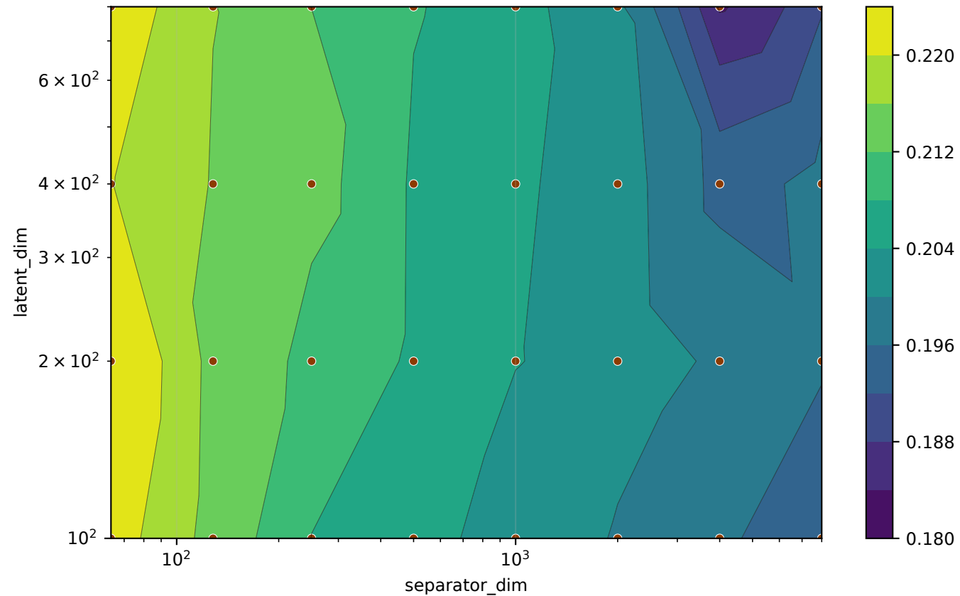
val/patterns_hoyer (steps=start..2000, last)
