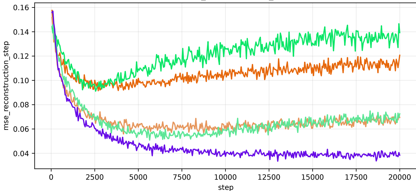
train/mse_reconstruction_step
