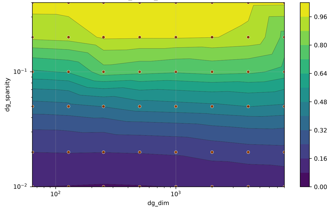
val/patterns_active_rate (steps=all, last)
