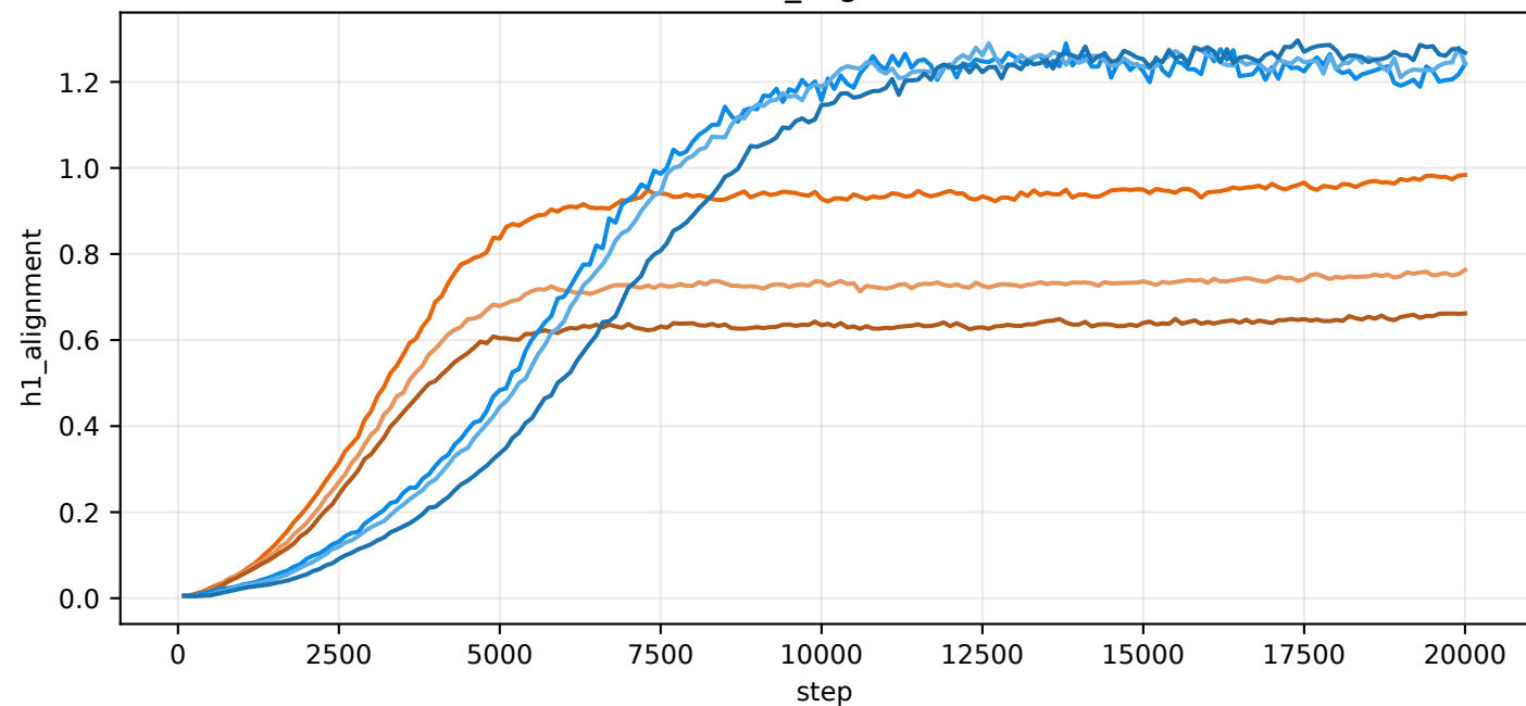
val/h1_alignment
