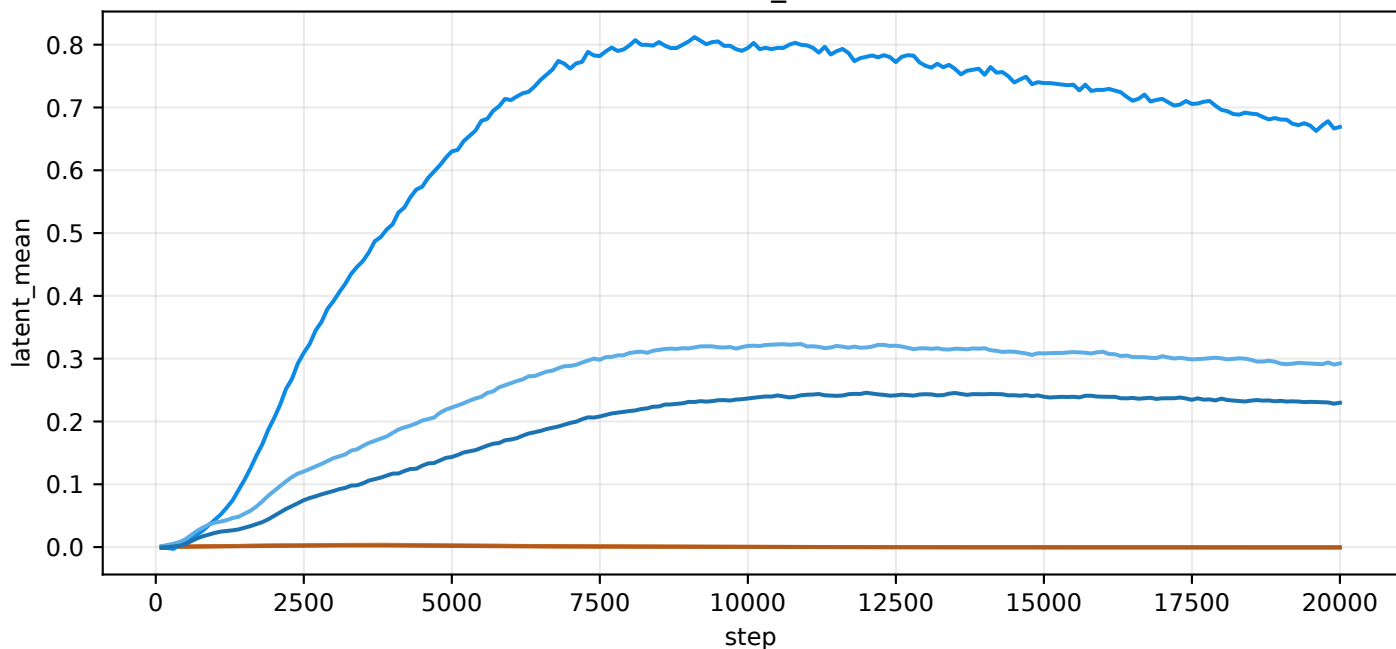
val/latent_mean
