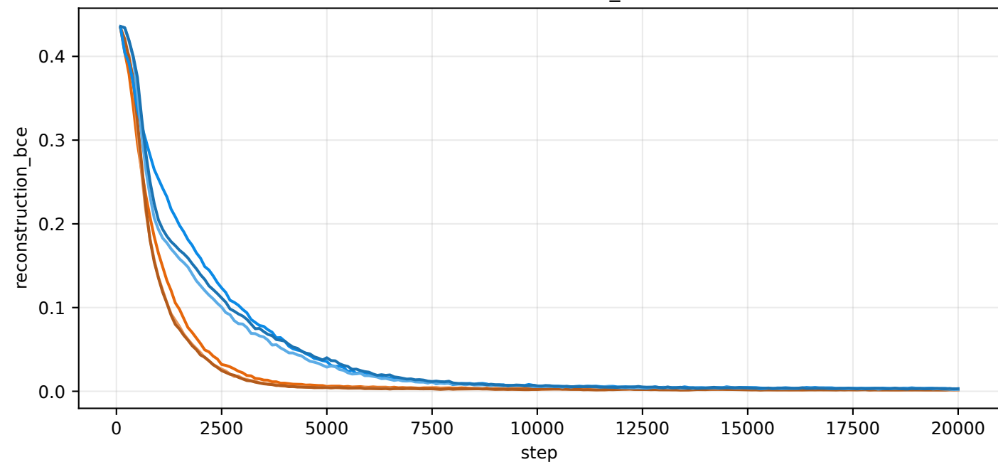
val/reconstruction_bce
