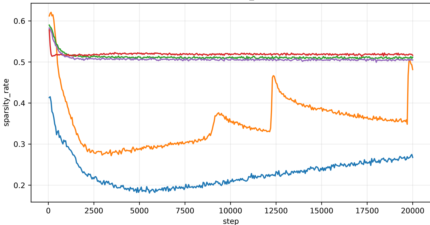
train/sparsity_rate
