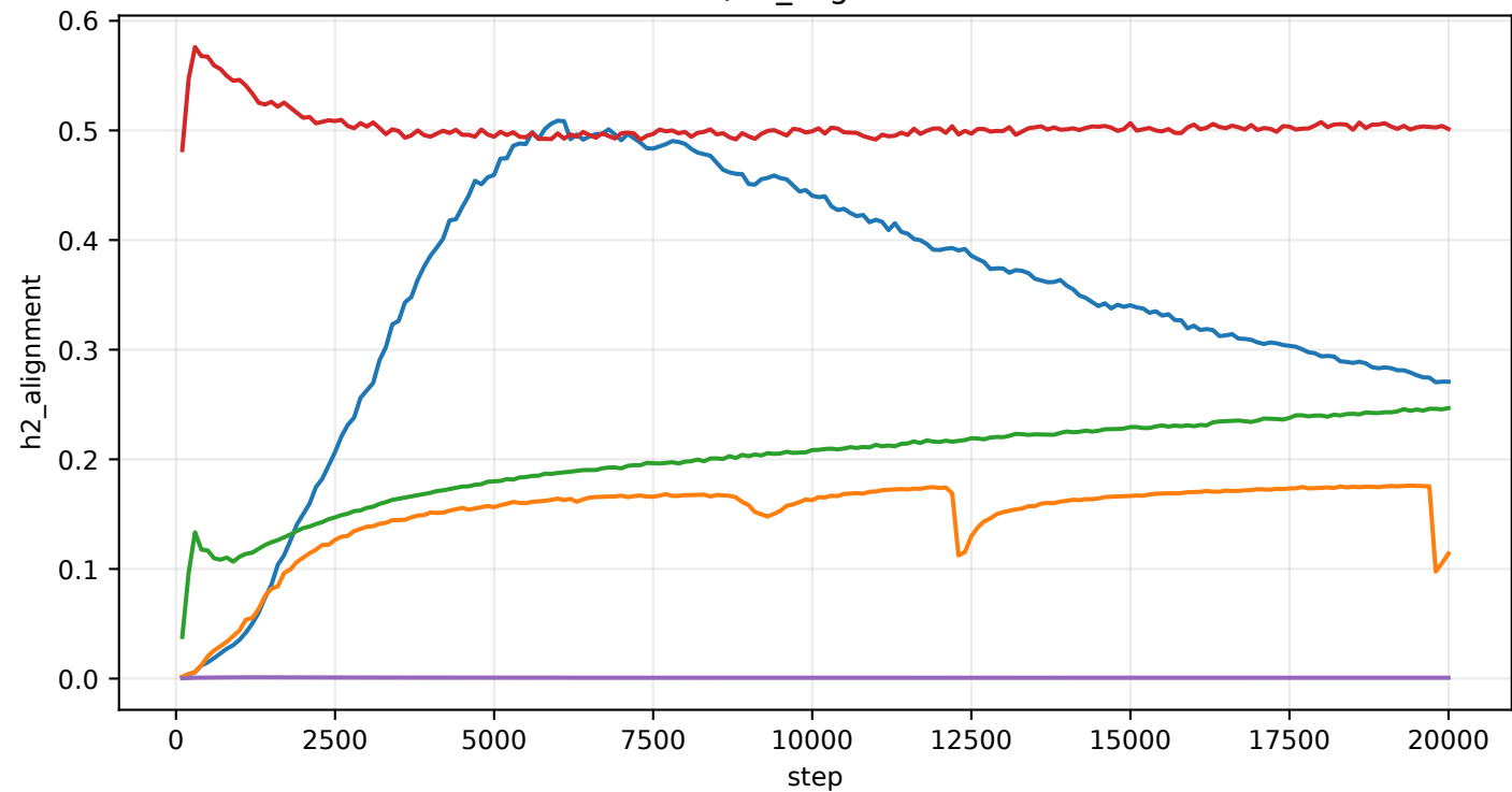
val/h2_alignment
