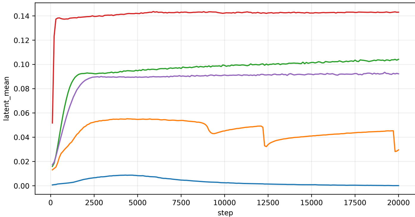
val/latent_mean
