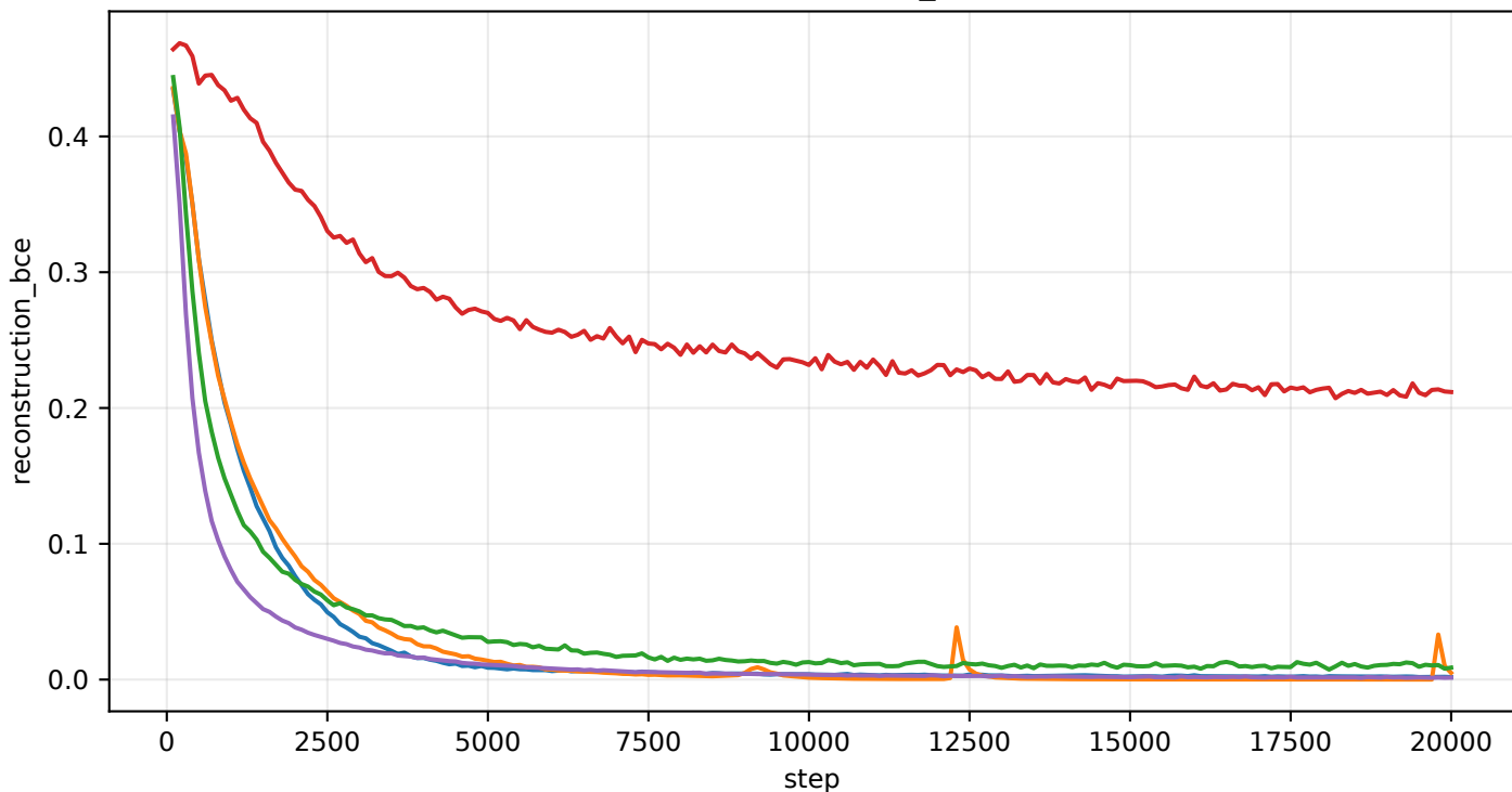
val/reconstruction_bce
