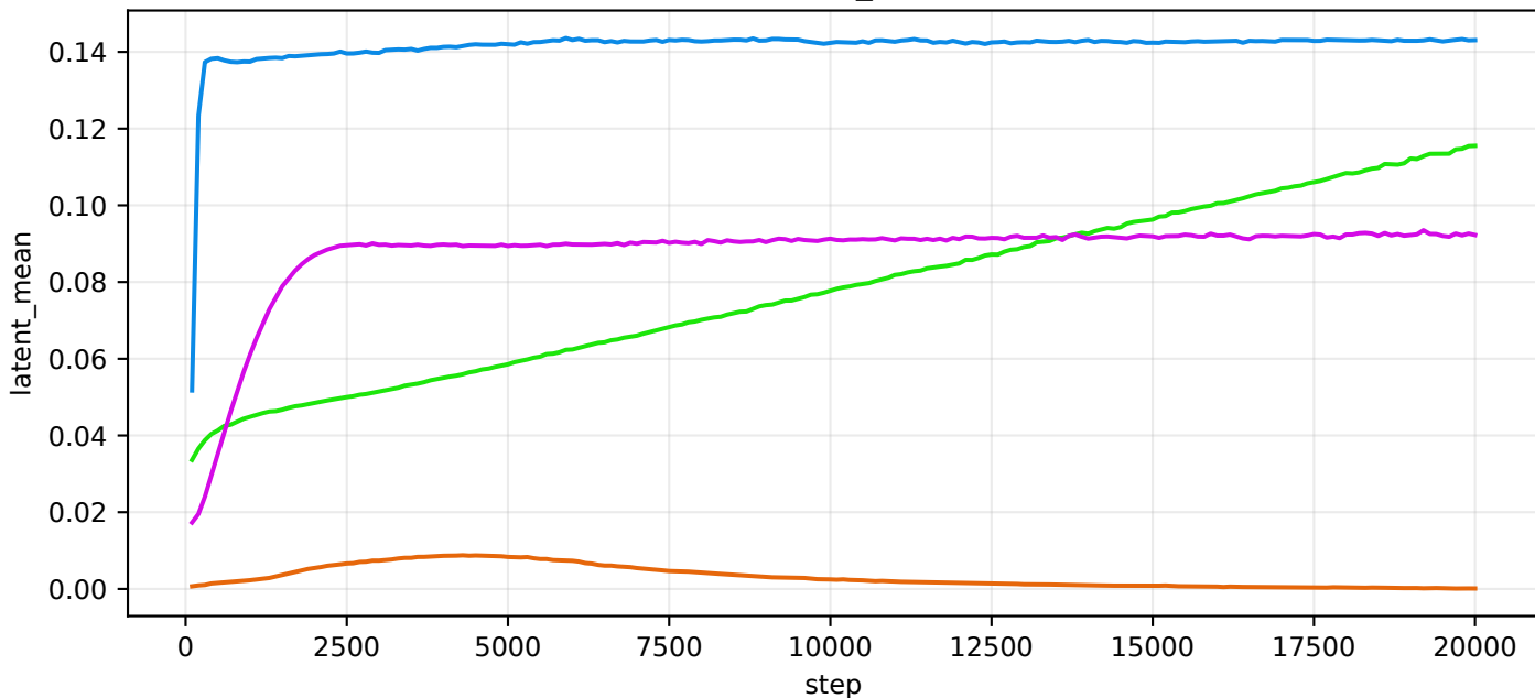
val/latent_mean
