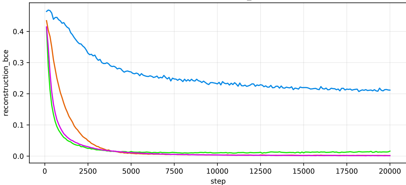
val/reconstruction_bce
