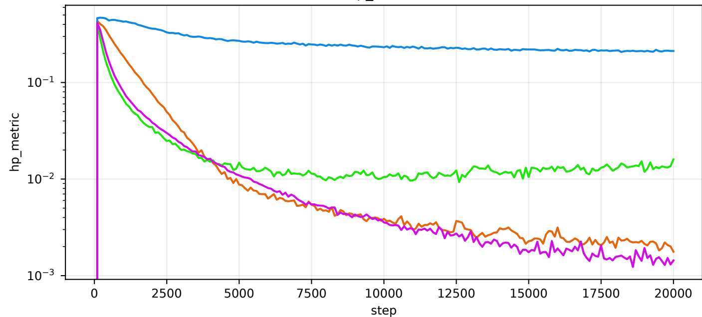
hp_metric
