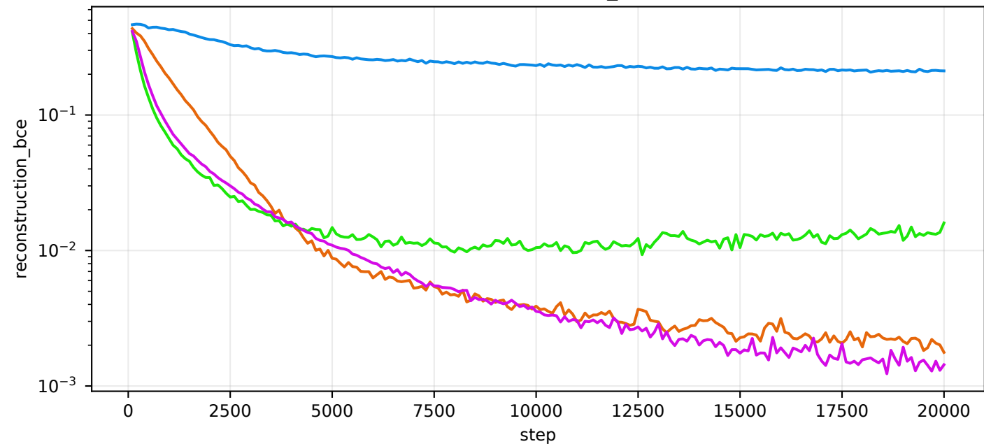
val/reconstruction_bce
