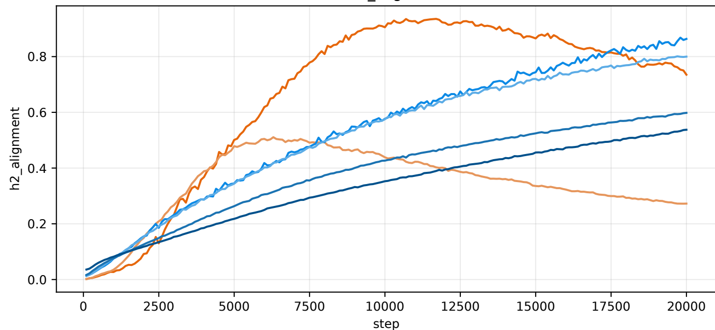
val/h2_alignment
