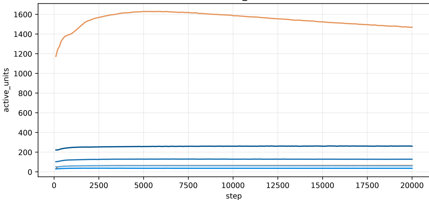
val/active_units
