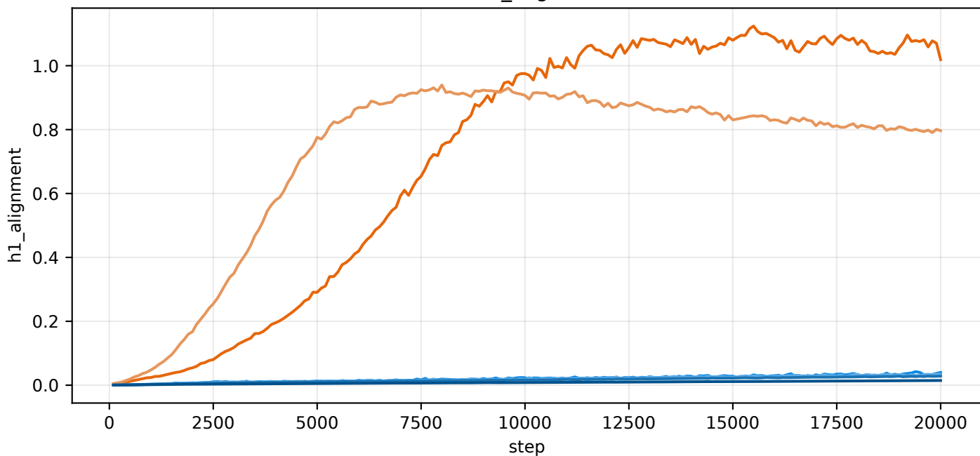
val/h1_alignment
