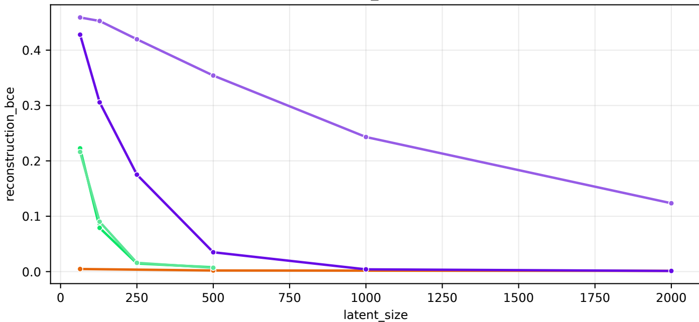
train/reconstruction_bce (steps=all, last)
