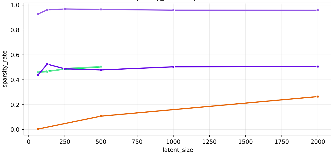
val/sparsity_rate (steps=all, last)
