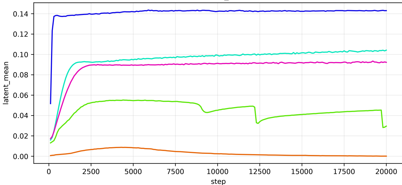
val/latent_mean
