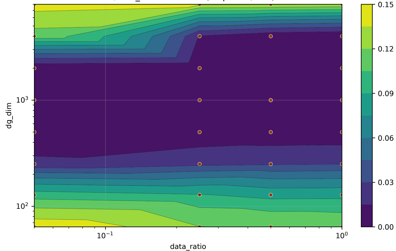
val/mse_reconstruction (steps=all, last)
