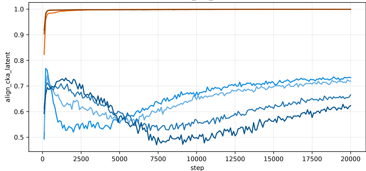
val/align_cka_latent
