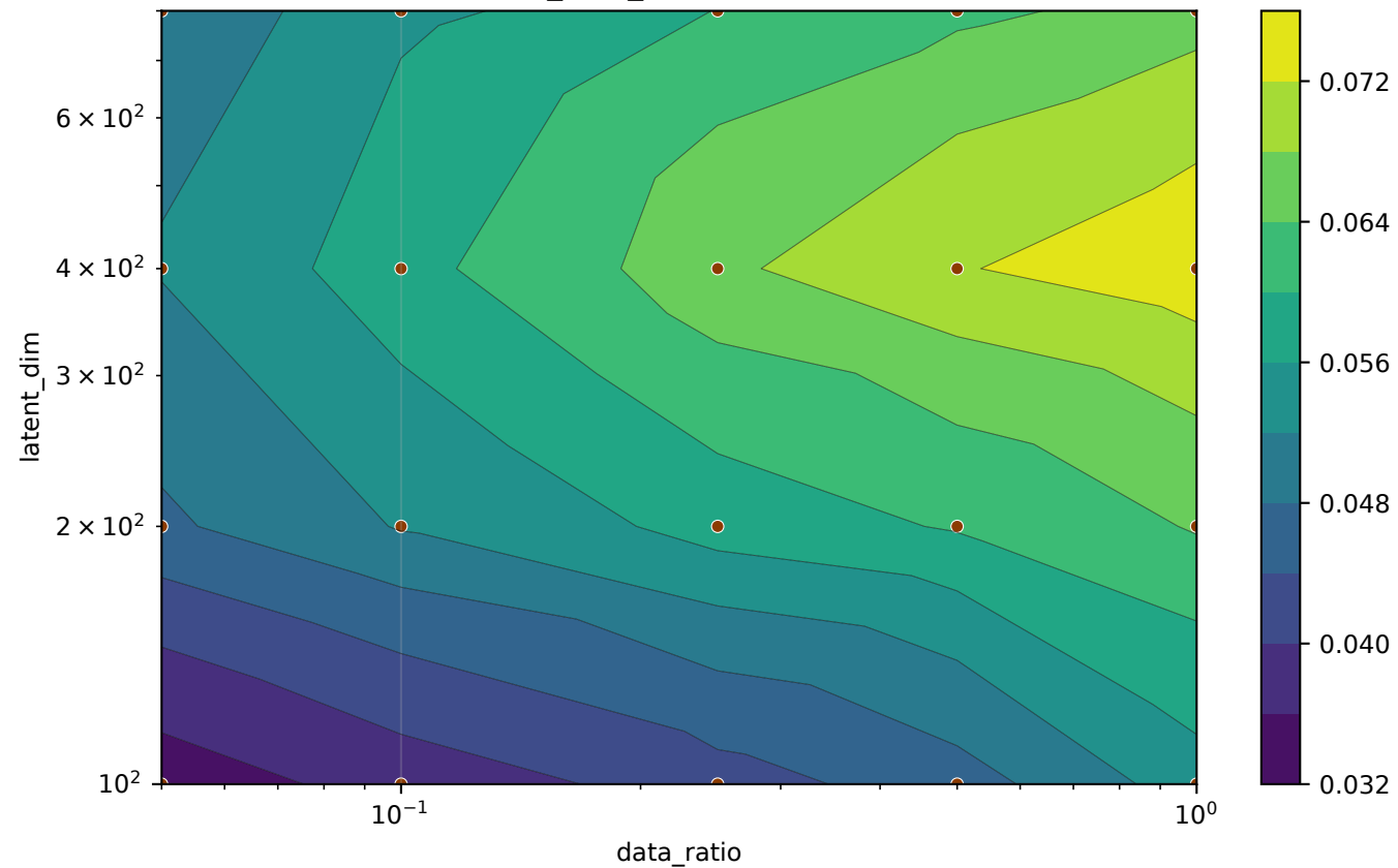
train/latent_post_hoyer (steps=all, last)
