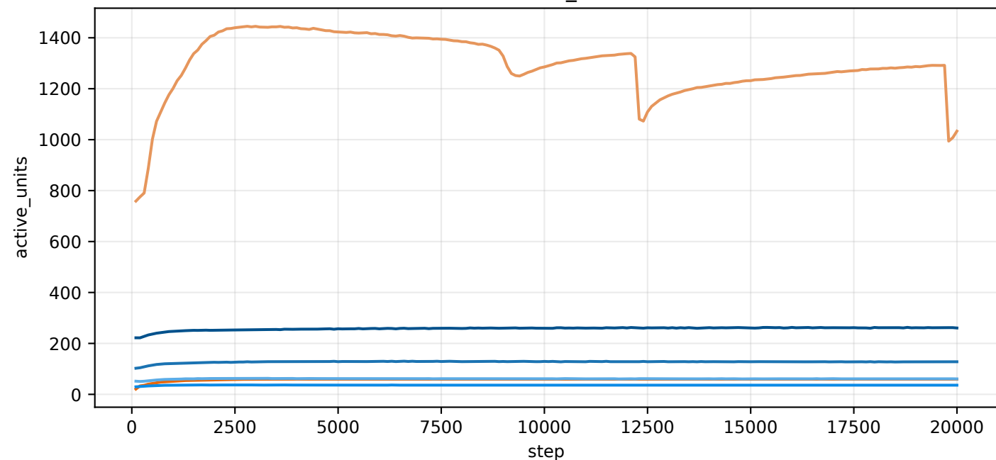
val/active_units
