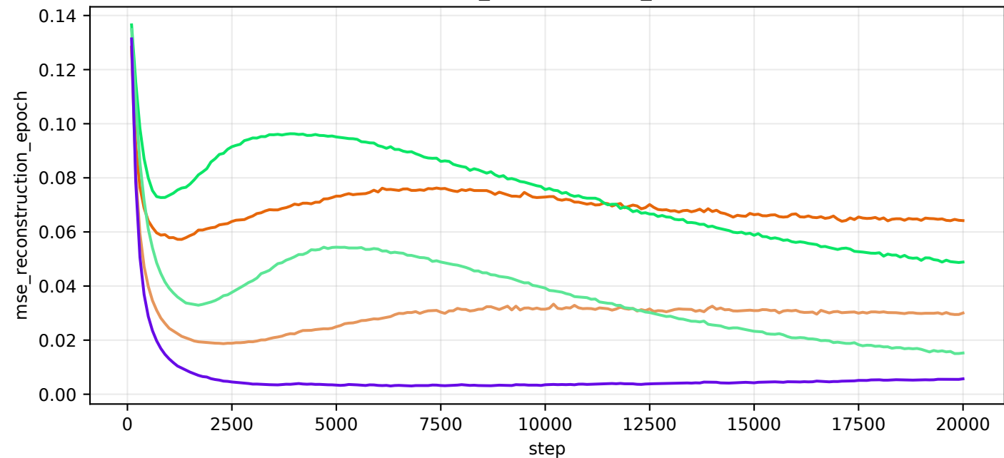
train/mse_reconstruction_epoch
