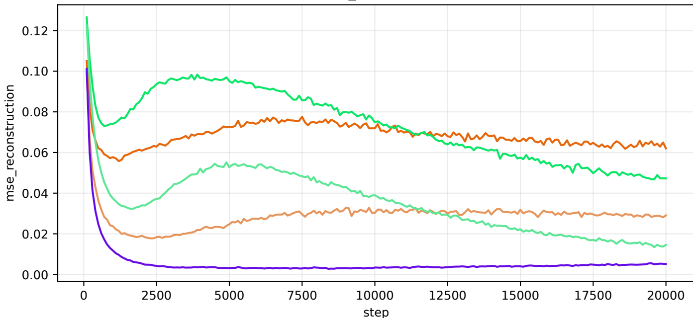
val/mse_reconstruction
