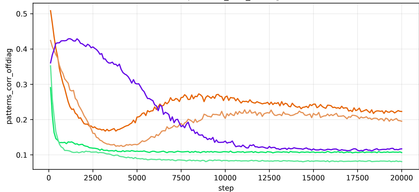
val/patterns_corr_offdiag
