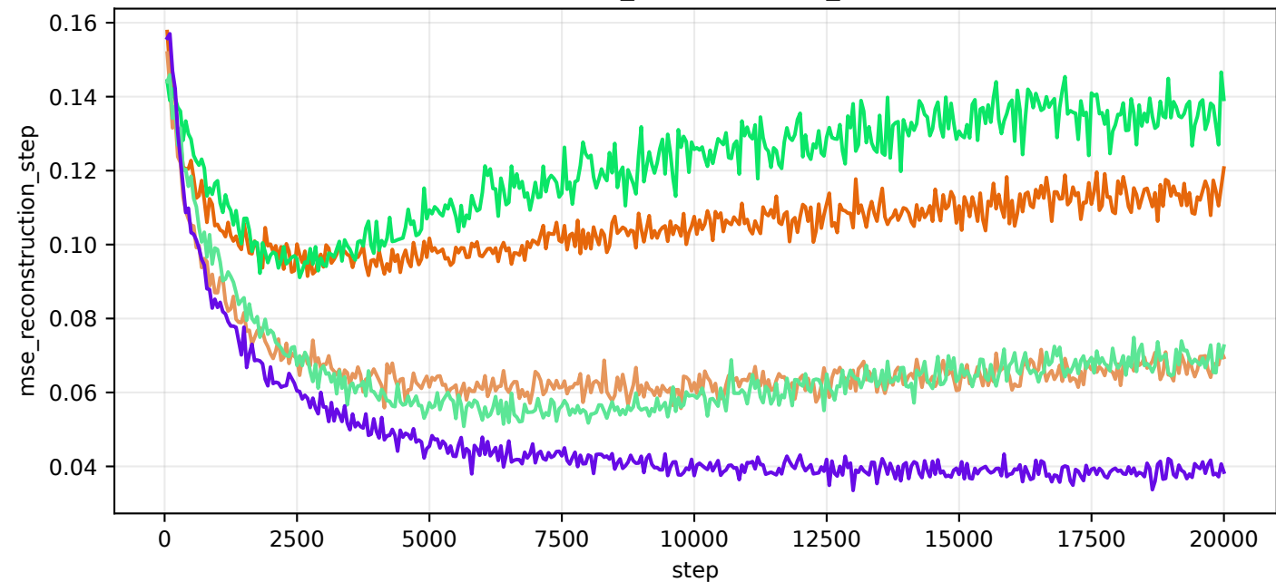
train/mse_reconstruction_step
