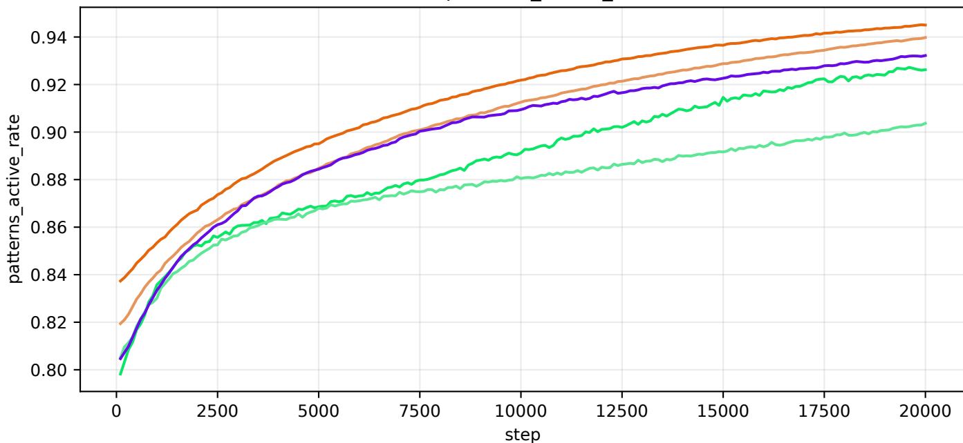
train/patterns_active_rate
