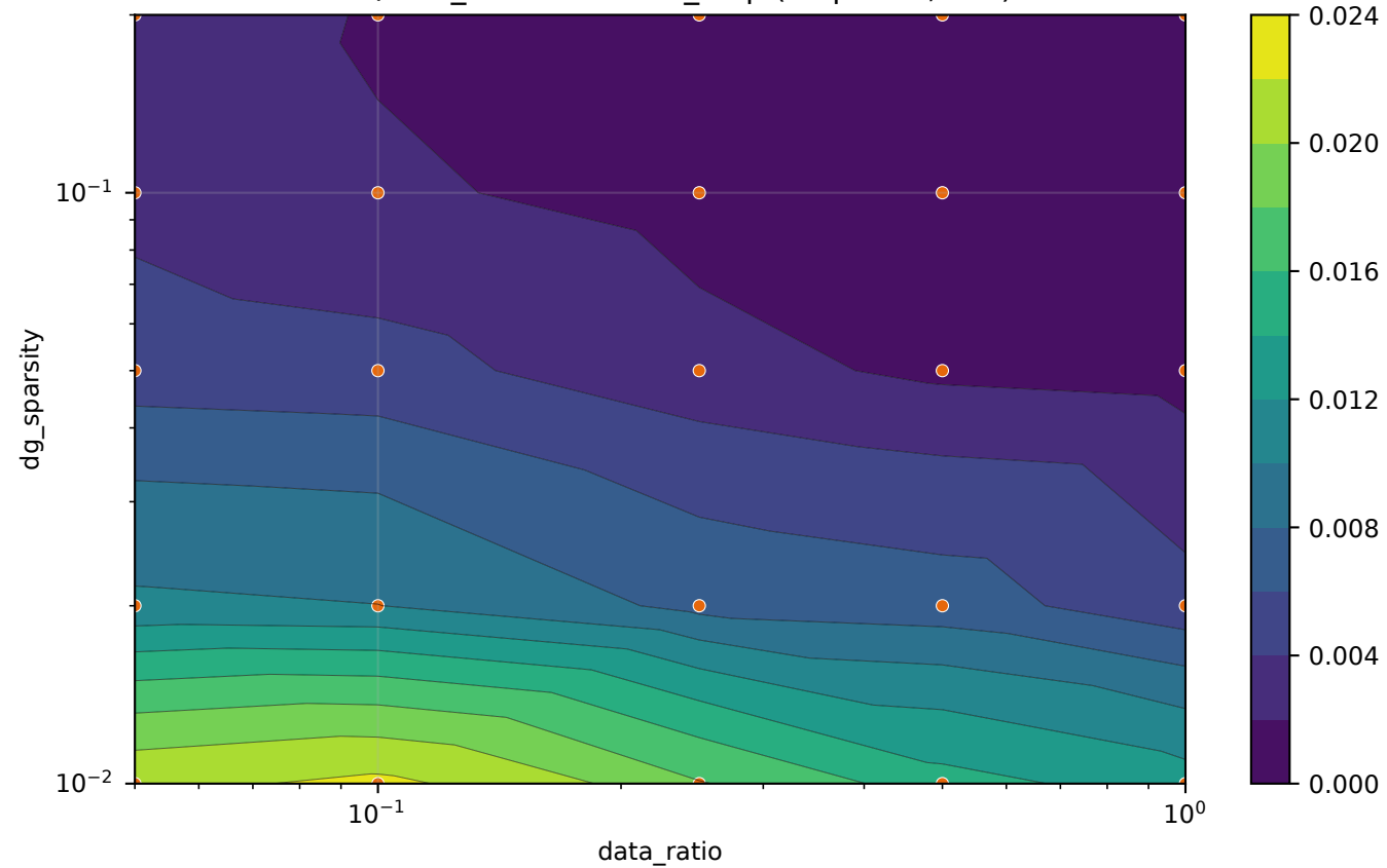
train/mse_reconstruction_step (steps=all, last)
