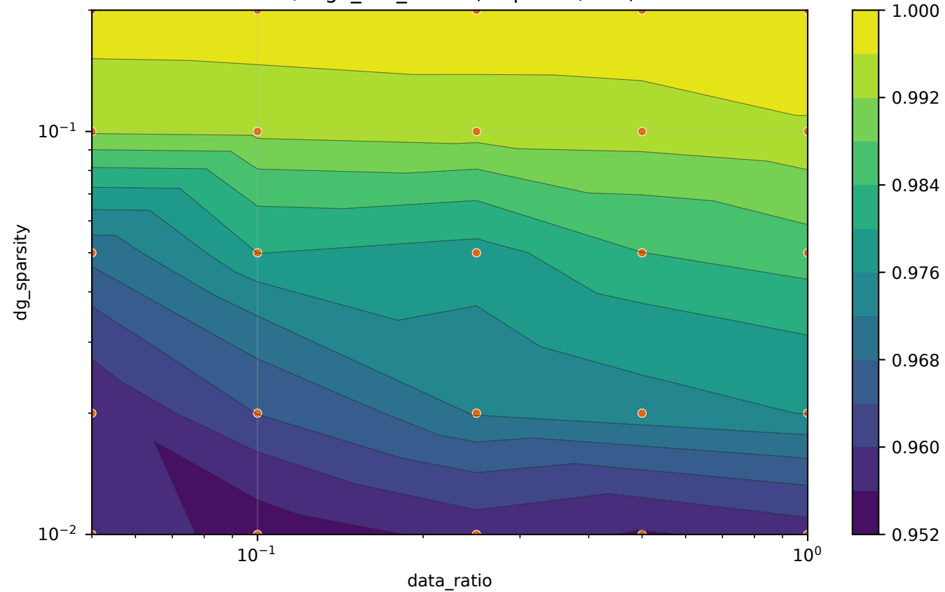
val/align_cka_latent (steps=all, last)
