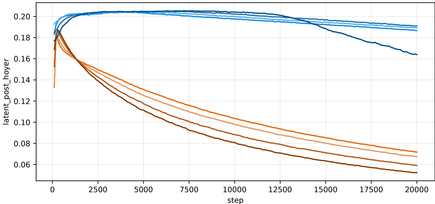
train/latent_post_hoyer
