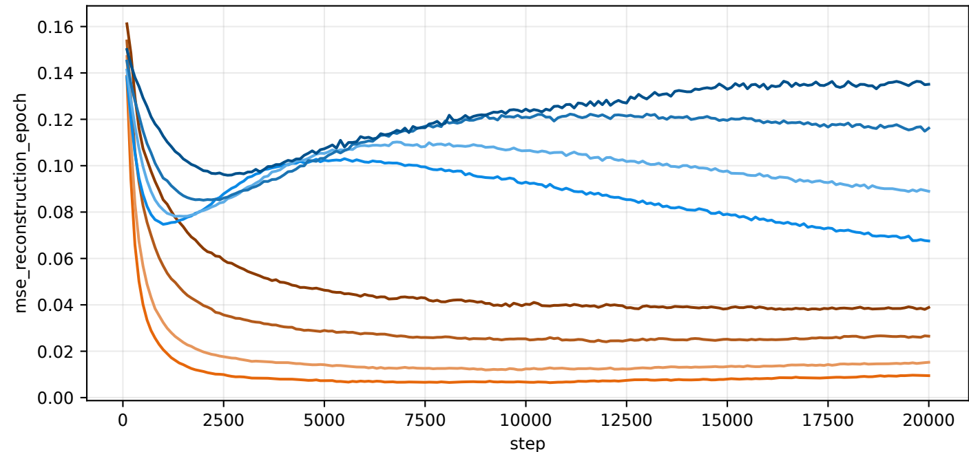
train/mse_reconstruction_epoch
