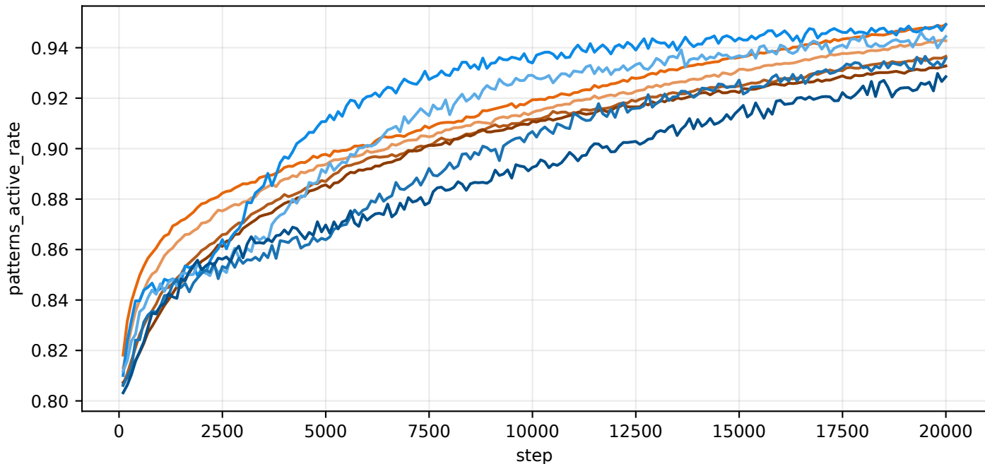
val/patterns_active_rate
