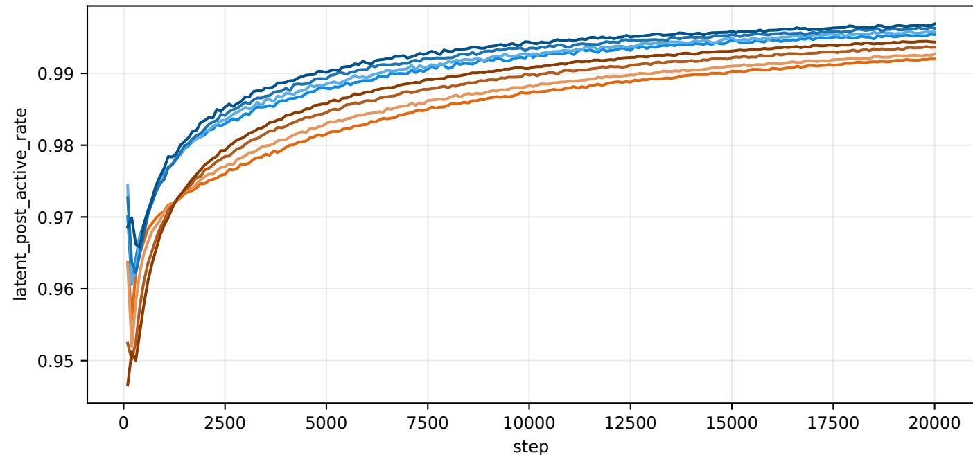
train/latent_post_active_rate
