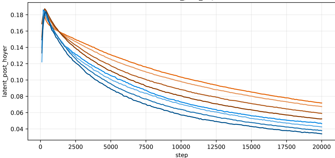
train/latent_post_hoyer
