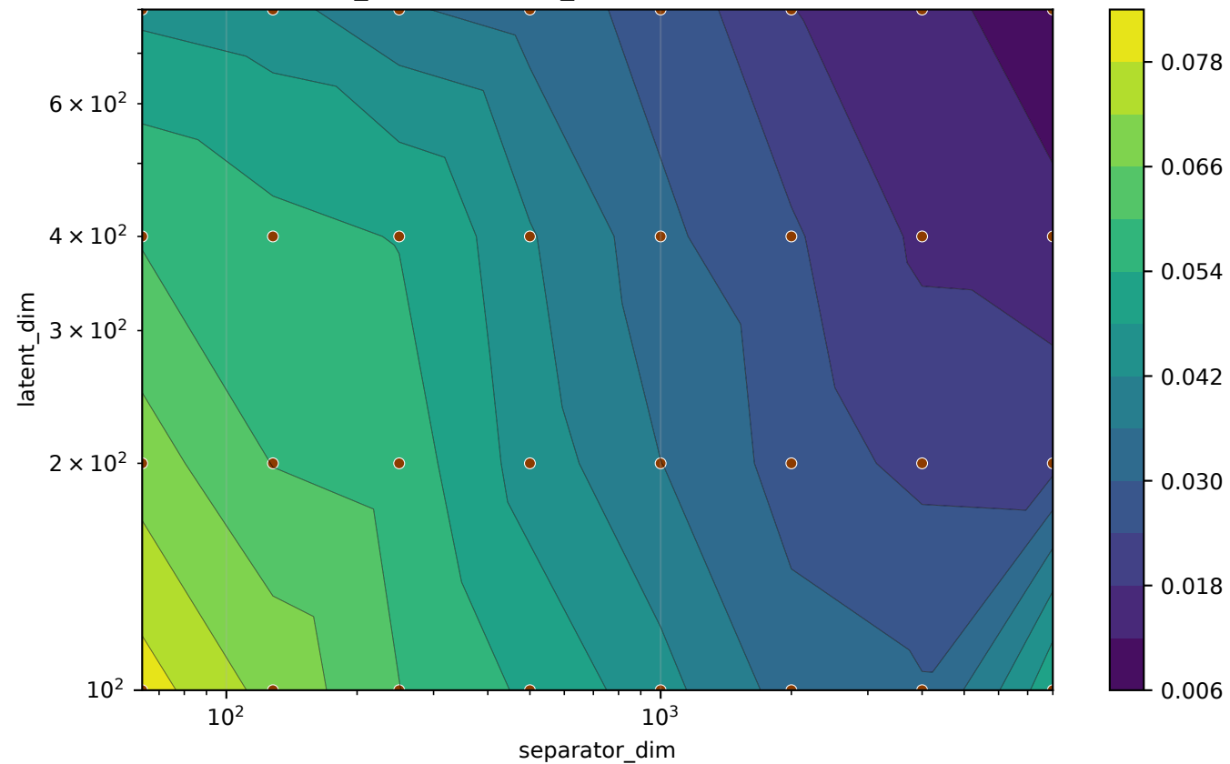
train/mse_reconstruction_step (steps=start..2000, last)
