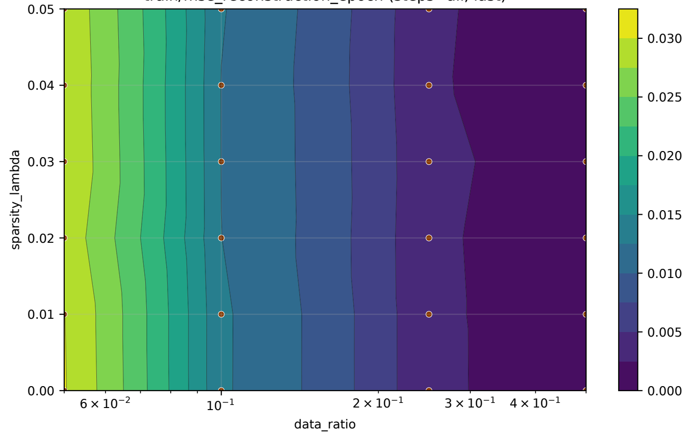
train/mse_reconstruction_epoch (steps=all, last)
