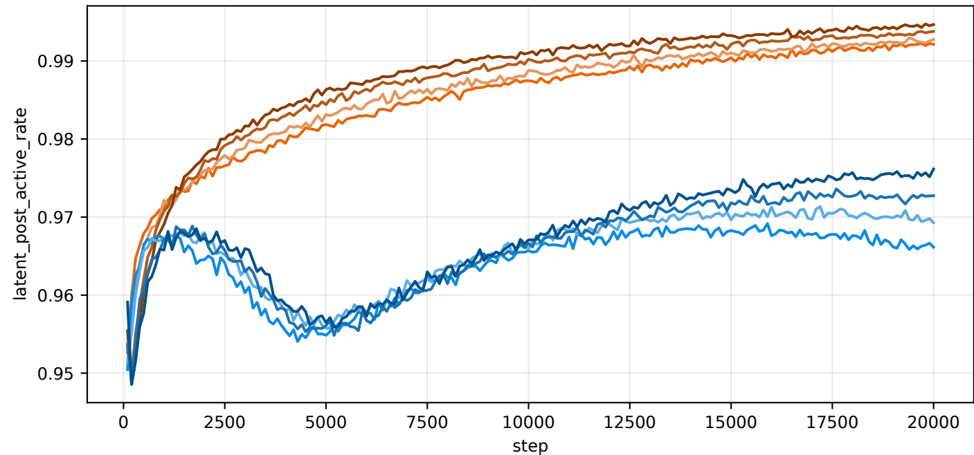
val/latent_post_active_rate
