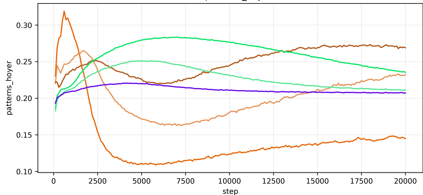
val/patterns_hoyer
