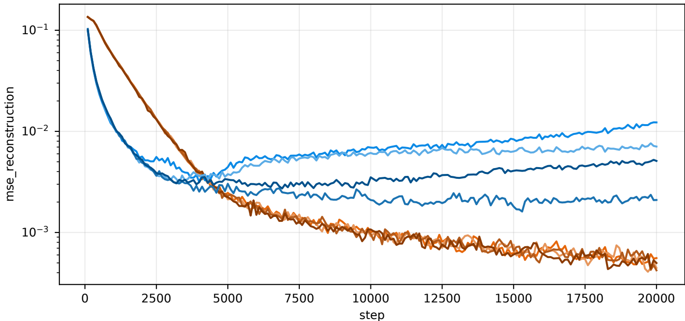
val/mse_reconstruction
