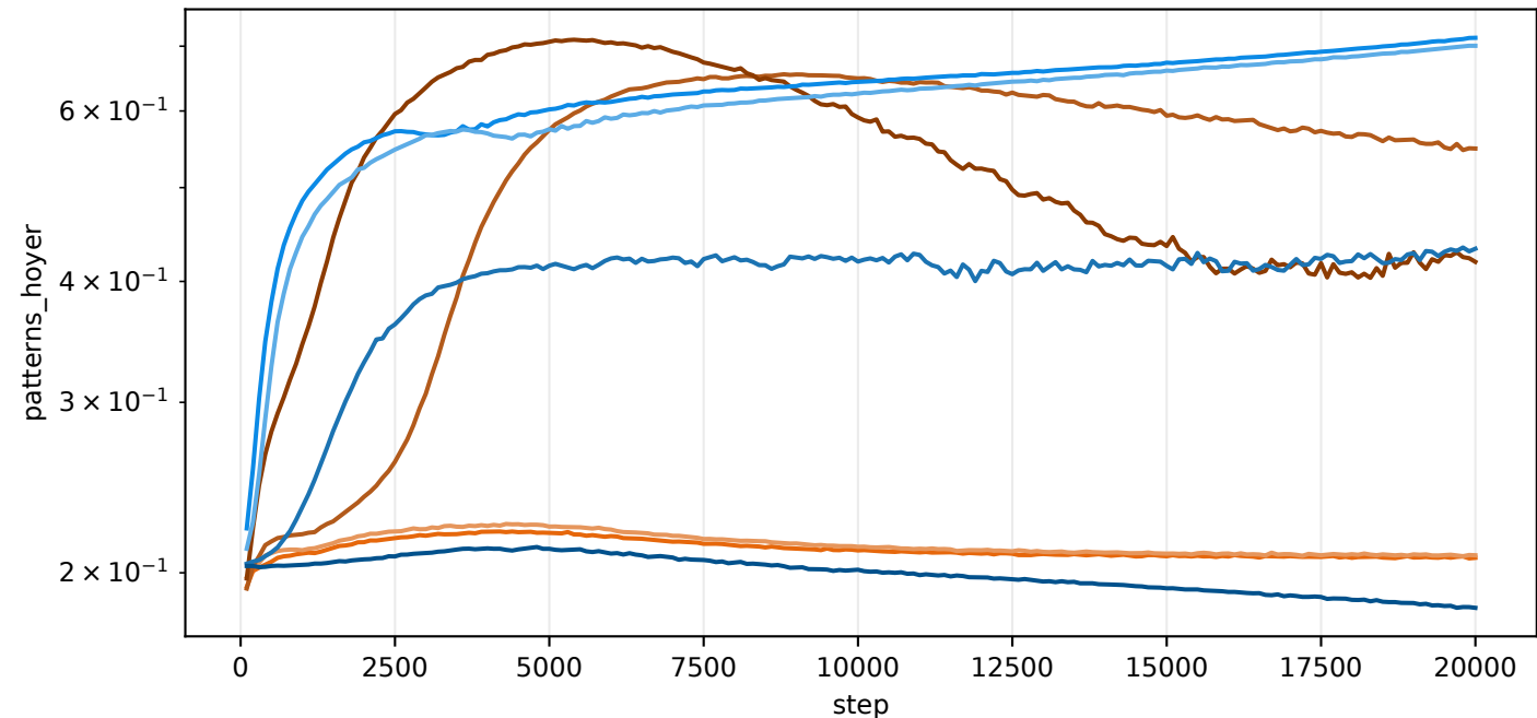
val/patterns_hoyer
