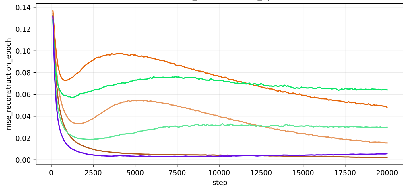
train/mse_reconstruction_epoch
