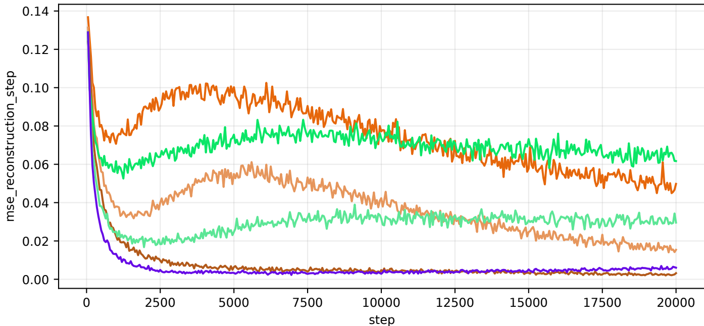
train/mse_reconstruction_step
