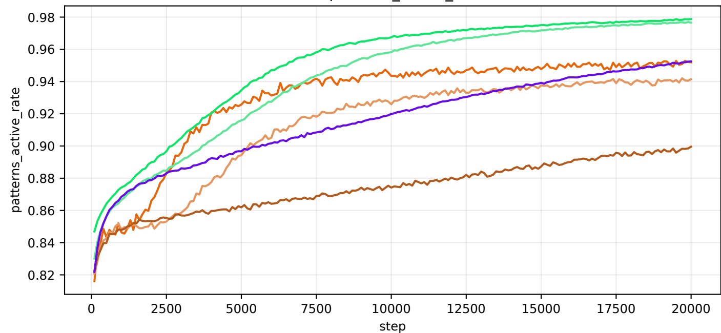
val/patterns_active_rate
