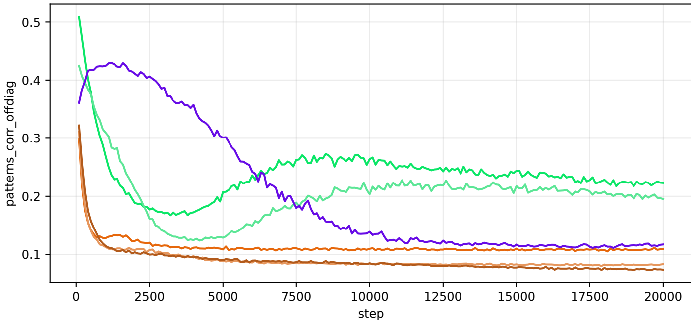
val/patterns_corr_offdiag
